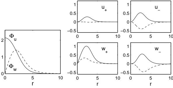
FIG. 5. The vortex soliton (left) and its unstable eigenmode (right) at s = 0.5 , \lambda = 0.5 and n = 2 . In the right figure, solid lines are the real parts of the eigenfunctions, and dashed lines are the imaginary parts.
